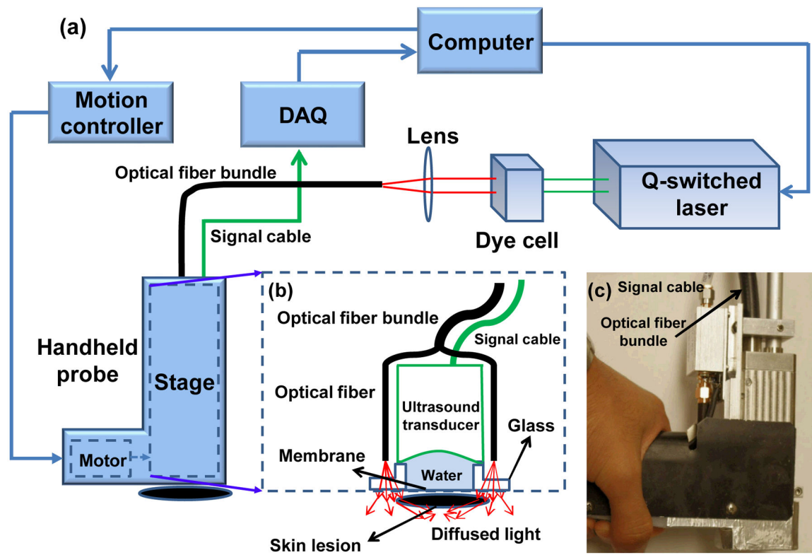
Fig. 1. Experimental handheld photoacoustic microscopy (PAM) system. (a) Schematic of the handheld PAM system. (b) Components held by the translation stage in the handheld probe. (c) A photograph of the handheld probe.
