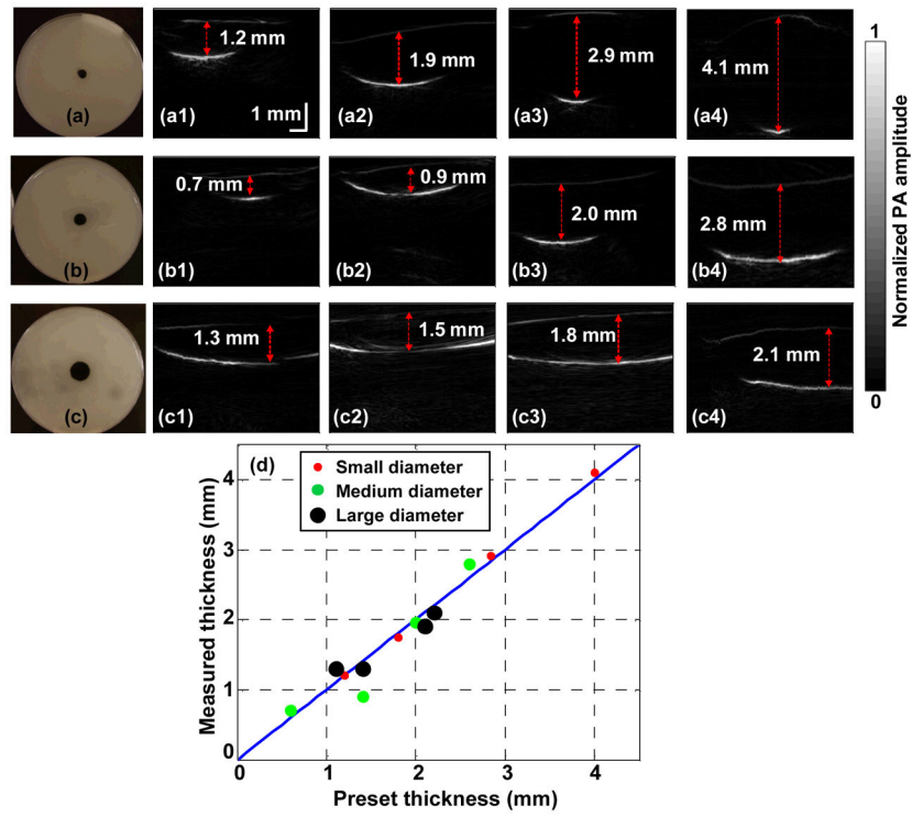
Fig. 4. Handheld PAM of melanoma phantoms. Photos of melanoma phantoms with different diameters ((a), 7 mm; (b), 9.5 mm; and (c), 14 mm). (a1–a4), (b1–b4), and (c1–c4): PAM images of different thicknesses of melanoma phantoms with the same diameter as in (a), (b), and (c), respectively. (d) Measured thicknesses of melanoma phantoms versus preset thicknesses.
