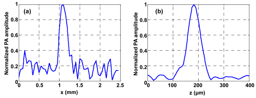
Fig. 3. Spatial resolutions of the current PAM system. PA amplitudes in the lateral x (a) and axial z (b) directions. The full widths at half maximum are 230 \mu\text{m} in (a) and 59 \mu\text{m} in (b).
