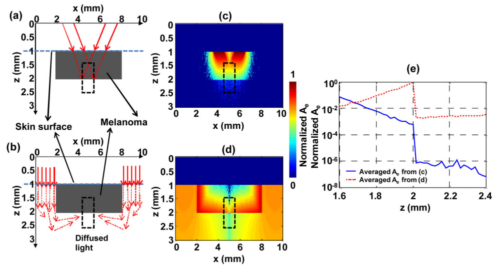
Fig. 2. Monte Carlo simulations of the old and new PAM systems for melanoma imaging. Melanoma phantom and light illumination methods used in the simulations of the old (a) and new (b) systems. The red arrows show the incident angles and areas of the light used in the Monte Carlo simulations. Specific heat absorption ( A_e ) distributions in the old (c) and new (d) PAM systems with the same incident energy. (e) Averaged A_e in the black-dashed-square areas (shown in (a–d)) at the bottom boundary of the melanoma phantoms in (c) (blue line) and (d) (red dotted line) showing that the melanoma is much more strongly illuminated at the bottom boundary using the new PAM system.
