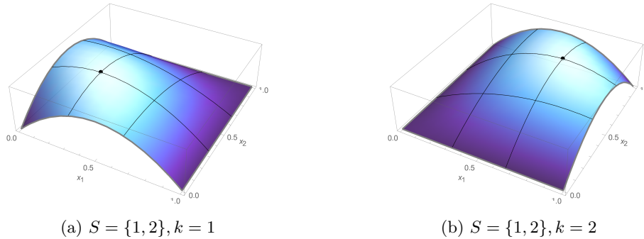
Fig. 1: Plot of h_S^k(x) for S = \{1, 2\} . The maximum is attained at x_1 = x_2 = 1/3 in (a) and at x_1 = x_2 = 2/3 in (b).
