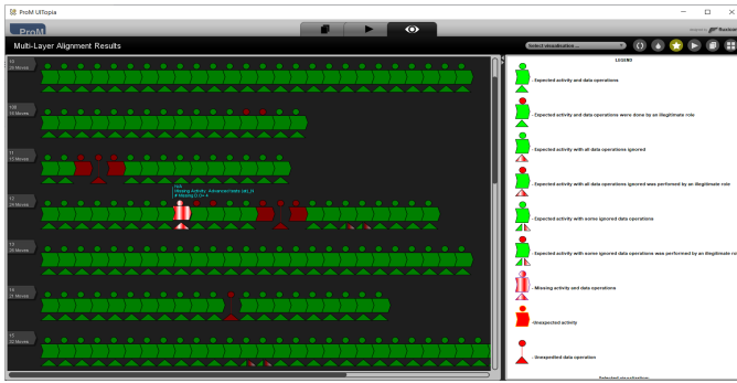
Fig. 1. Screenshot of the MLA Tool- Projection to process log visualisation
