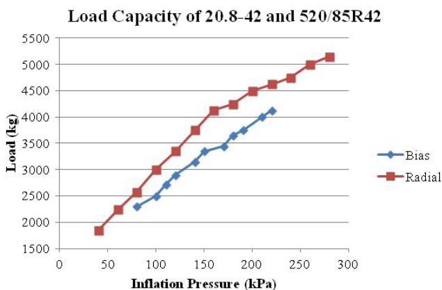
Figure 2. Graphical view of load table for 20.8-42 and 520/85R42 tires (from Tire and Rim Association, Inc., 2016 Year Book).
