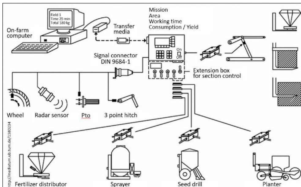
Figure 3: Applications of the mobile agricultural computer (centralized control, monitoring, closed-loop-control).
