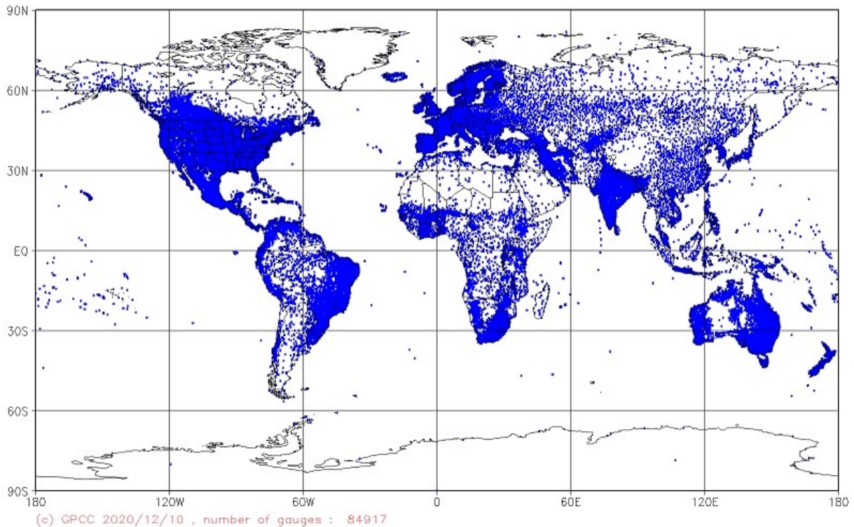
Figure 10: Spatial distribution of monthly in-situ stations with a climatological precipitation normal, based on at least 10 years of data in GPCC's database (number of stations in July: 84,917)
