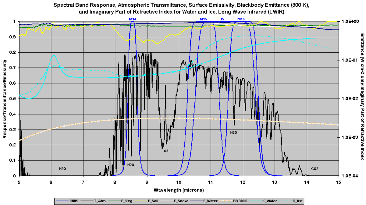
Figure 3. Phenomenology of the VIIRS LWIR Bands
