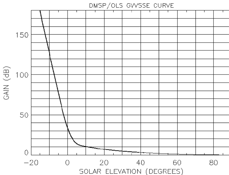
Figure 13. Typical GVVSSE curve for OLS on board variable gain control. The curve is designed so that a source with an albedo = 0.8 produces a 5 volt output signal from the analog signal processor.
