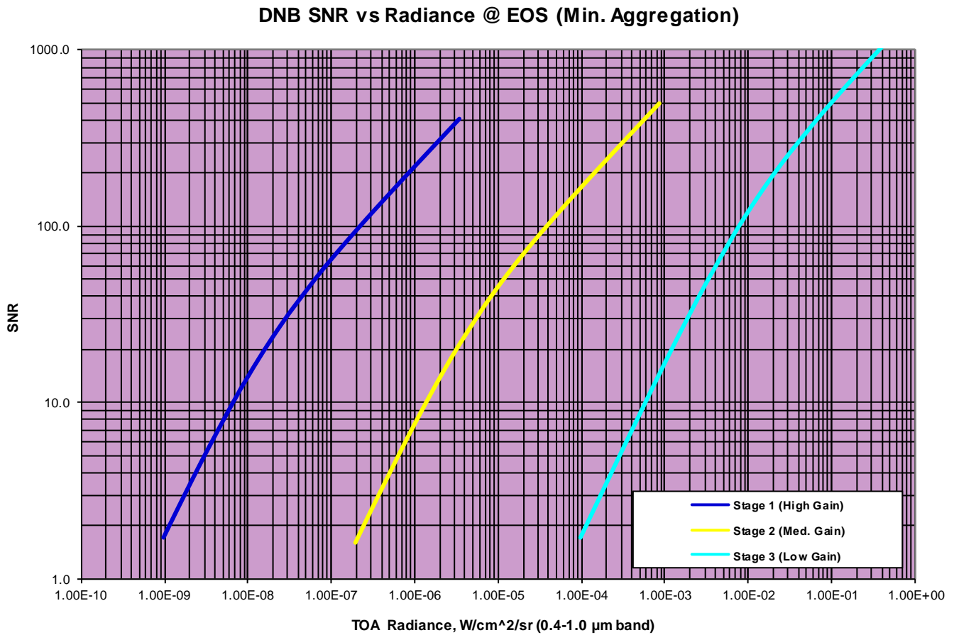
Figure 10. SNR performance for the DNB at edge-of-scan for each of the three CCD gain stages. SNR performance over the specified measurement range ( 4.0E-9 - 3.0E-2 W \cdot cm^{-2} \cdot sr^{-1} ) is 7 to 250. SNR greater than 3 is achieved at a radiance as low as 1.8E-9 .
