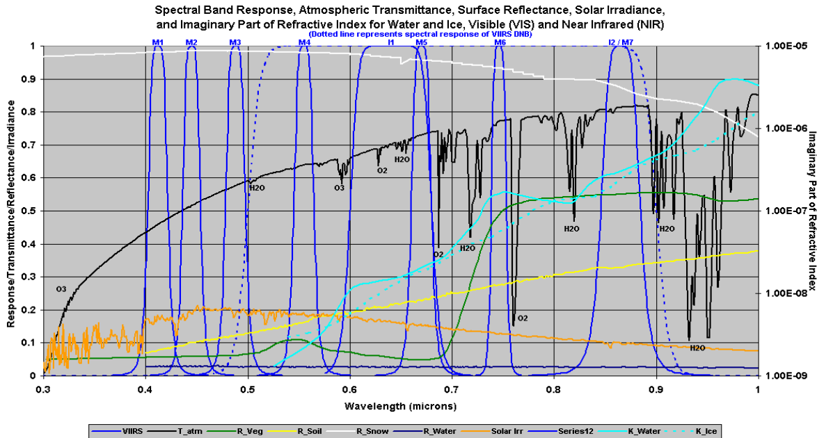
Figure 2. Phenomenology of the VIIRS Visible Bands
