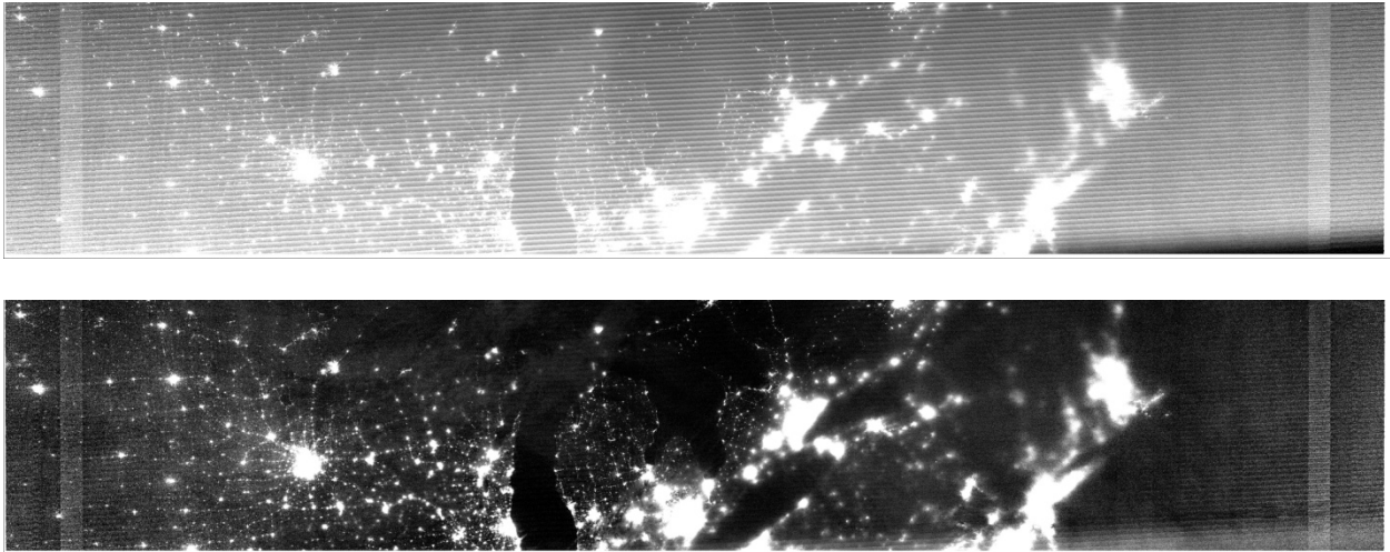
Figure 16. NCC Imagery taken over the United States Upper Midwest on 9 August 2013. The top portion of the figure is how the NCC Imagery would appear without the stray light correction in the DNB SDR, the lower image is after the stray light correction is applied.
