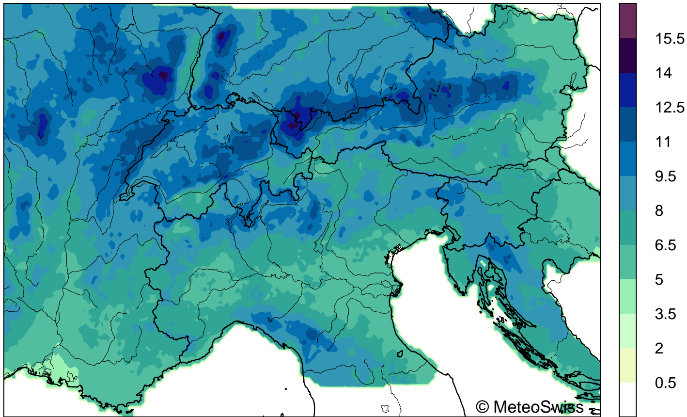
Maximum no. of consecutive wet days ([d],CWD), mean 197101–200812
