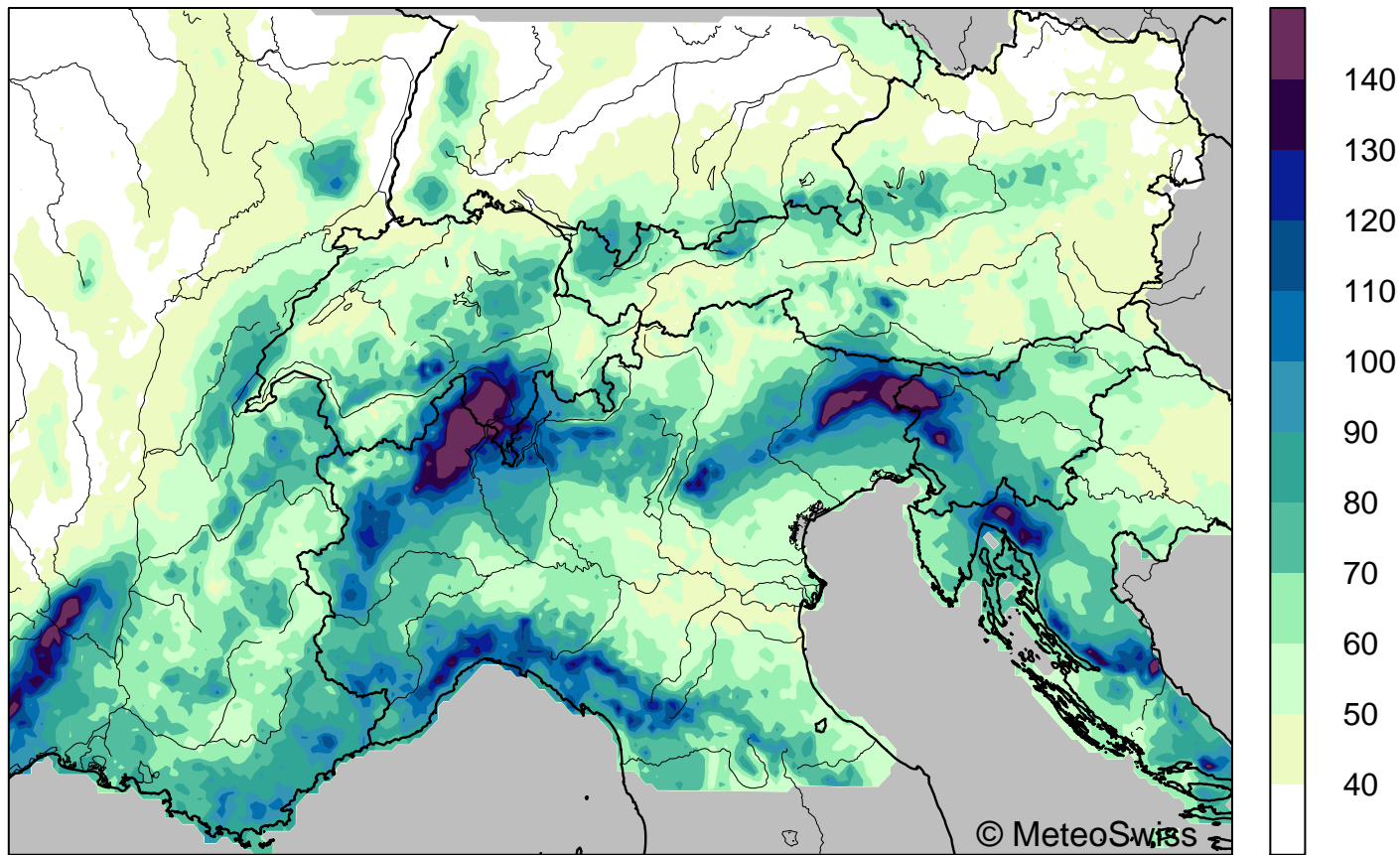
Highest 5-day precipitation amount ([mm],RX5day), mean 197101–200812
