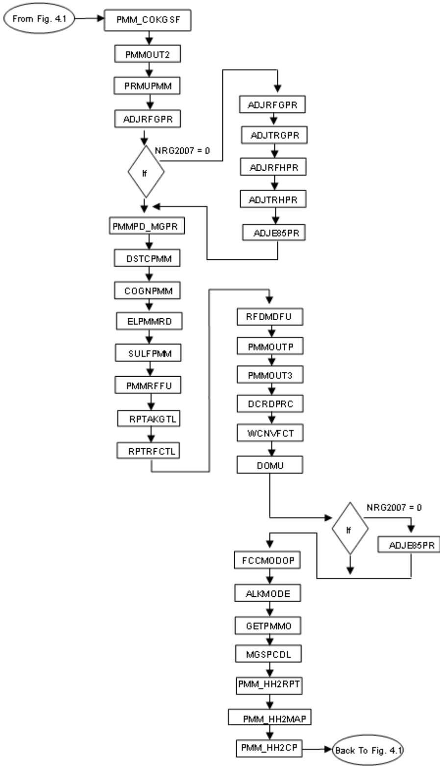
Figure 4.3 Matrix Postprocessing Subroutines
