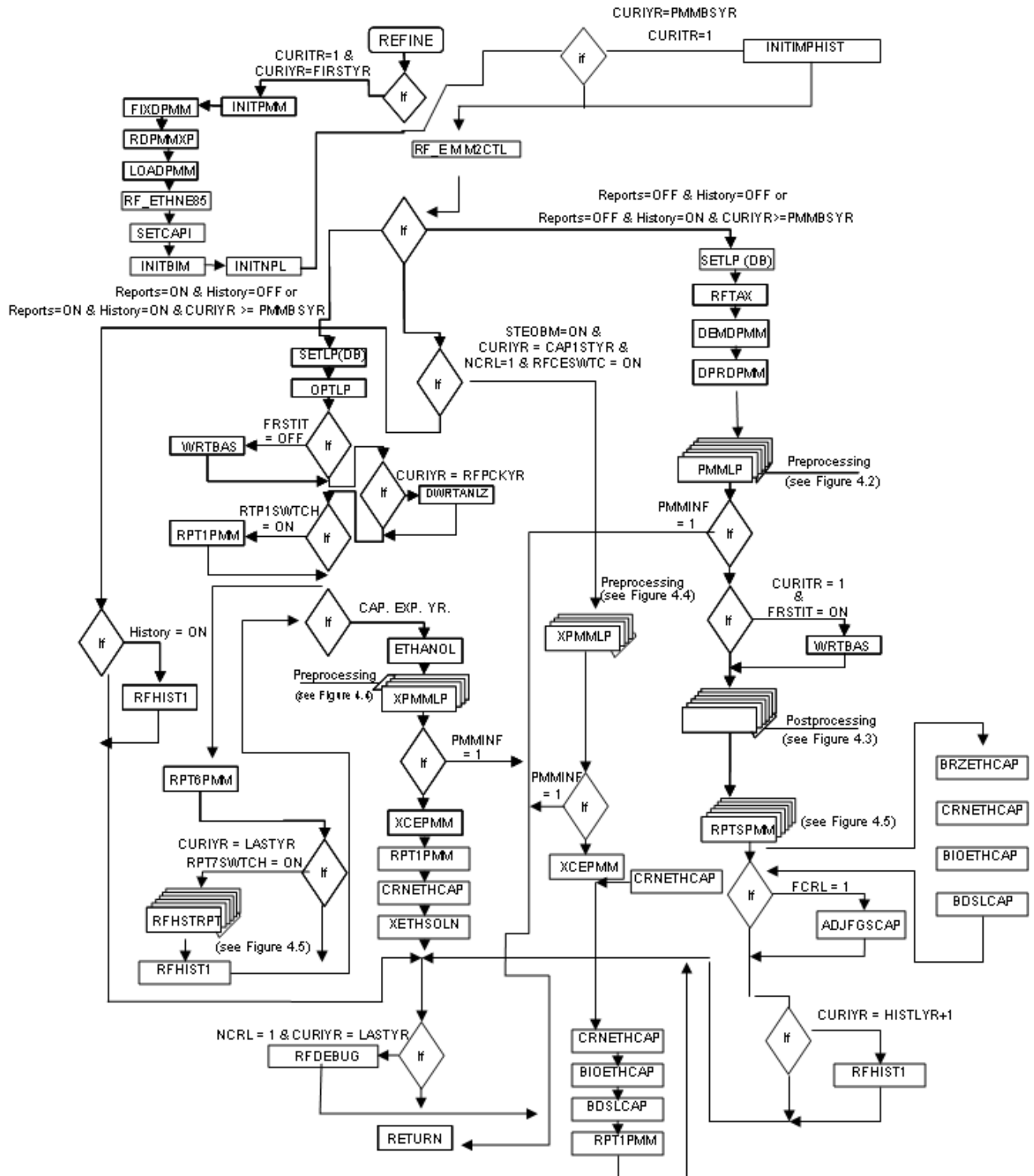
Figure 4.1 PMM Flow Diagram
