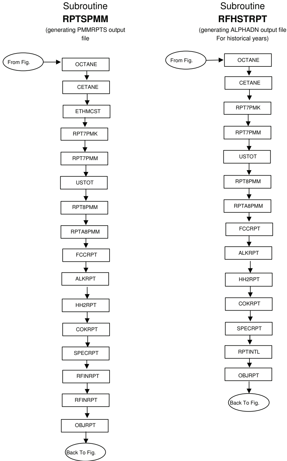
Figure 4.5 Report Subroutines
