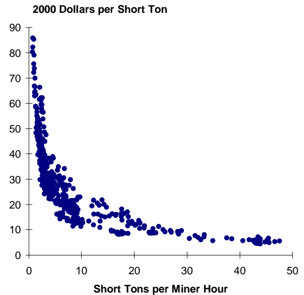
Figure 4. Minemouth Coal Prices and Labor Productivity for CMM Regions and Mine Types, 1978-2005
