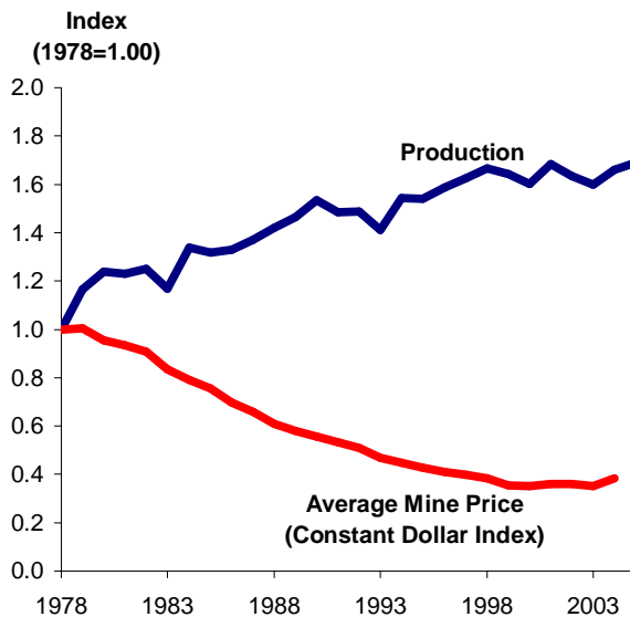
Figure 3. U.S. Coal Production and Prices, 1978-2005
