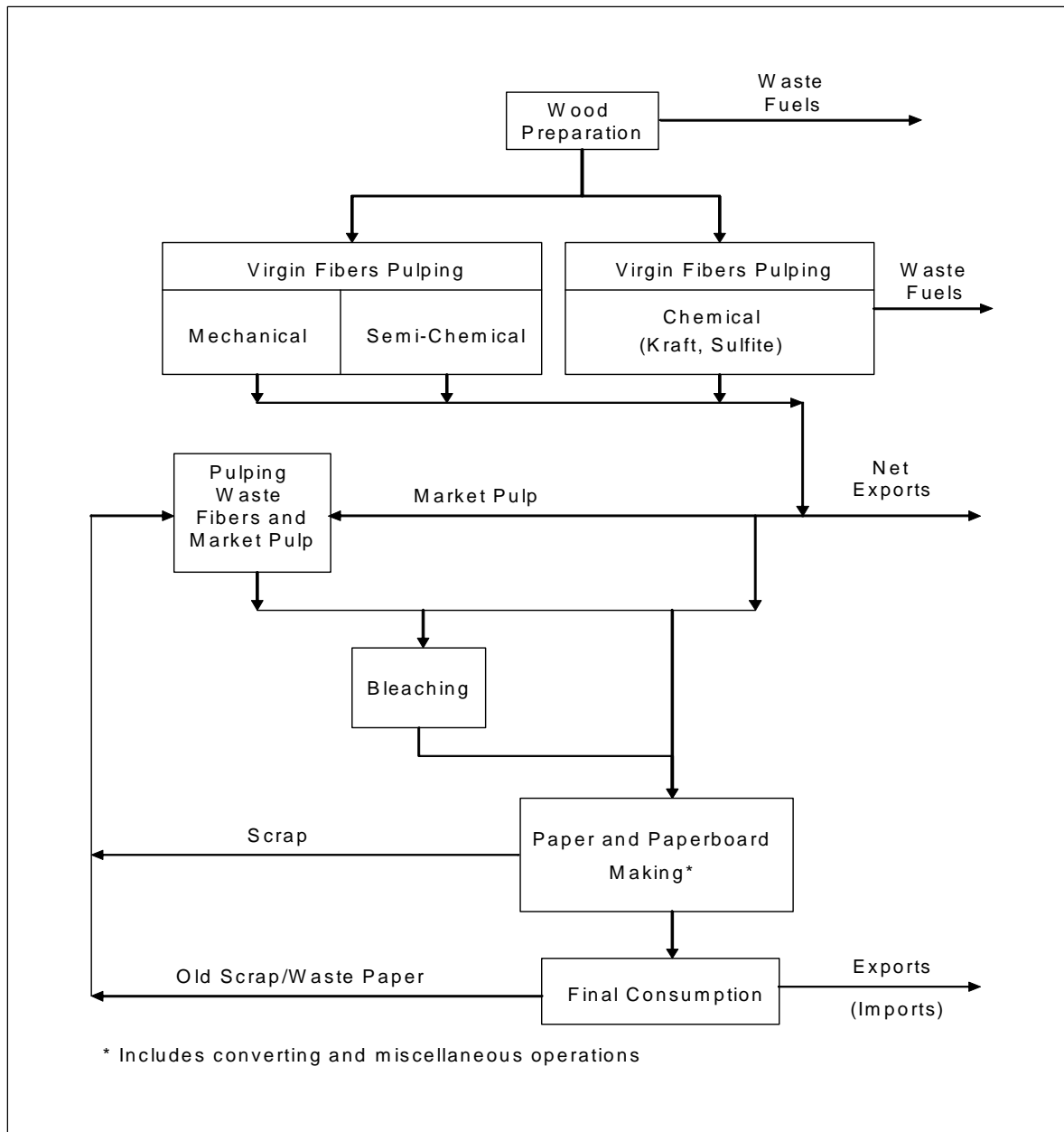
Figure 3. Paper Manufacturing Industry Process Flow
