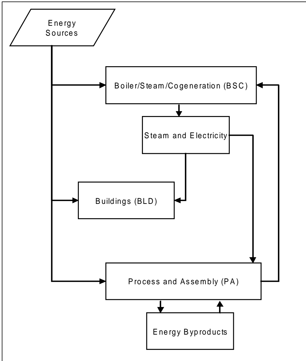
Figure 1. Industrial Module Components
