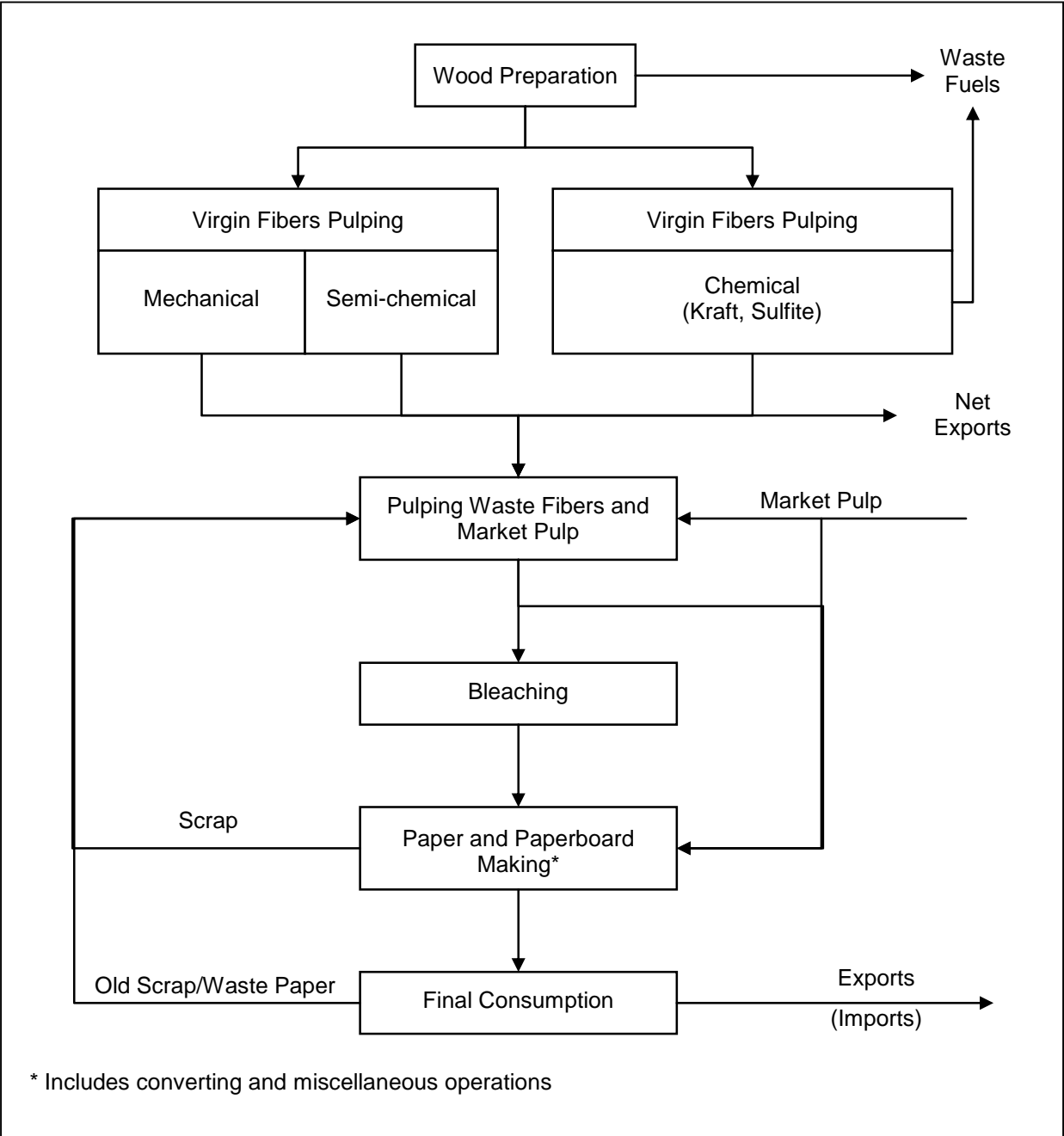
Figure 3. Paper Manufacturing Industry Process Flow
