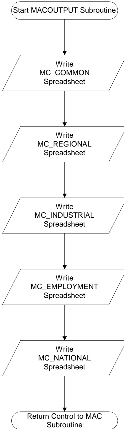
Figure 16. Subroutine MACOUTPUT
