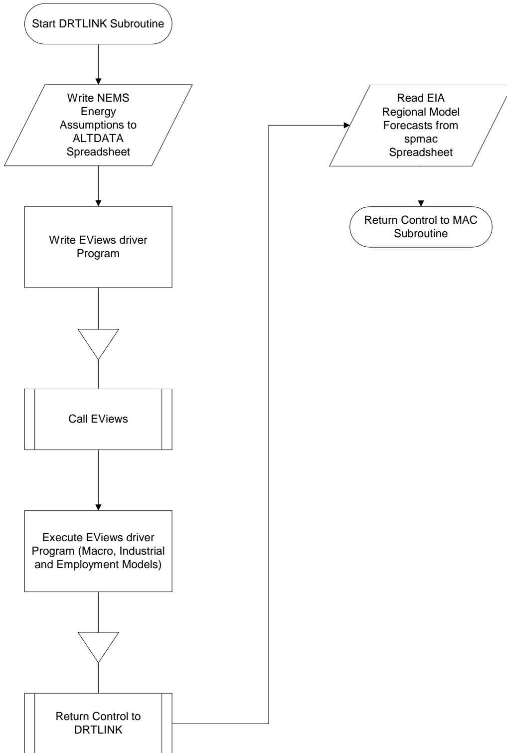
Figure 10. Subroutine DRTLINK
