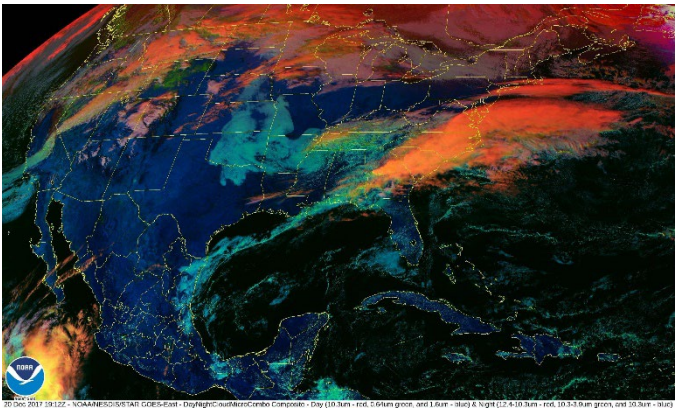
Sample product images for DayNightCloudMicroCombo over CONUS from March 2017 – January 2018.
