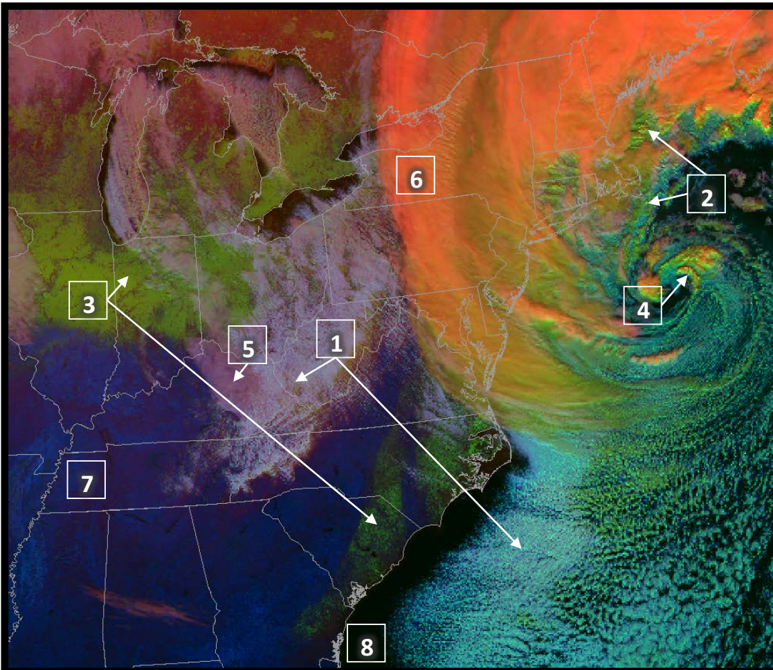
Day Cloud Phase Distinction RGB from GOES-16 ABI at 1735 UTC, 04 January 2018.
